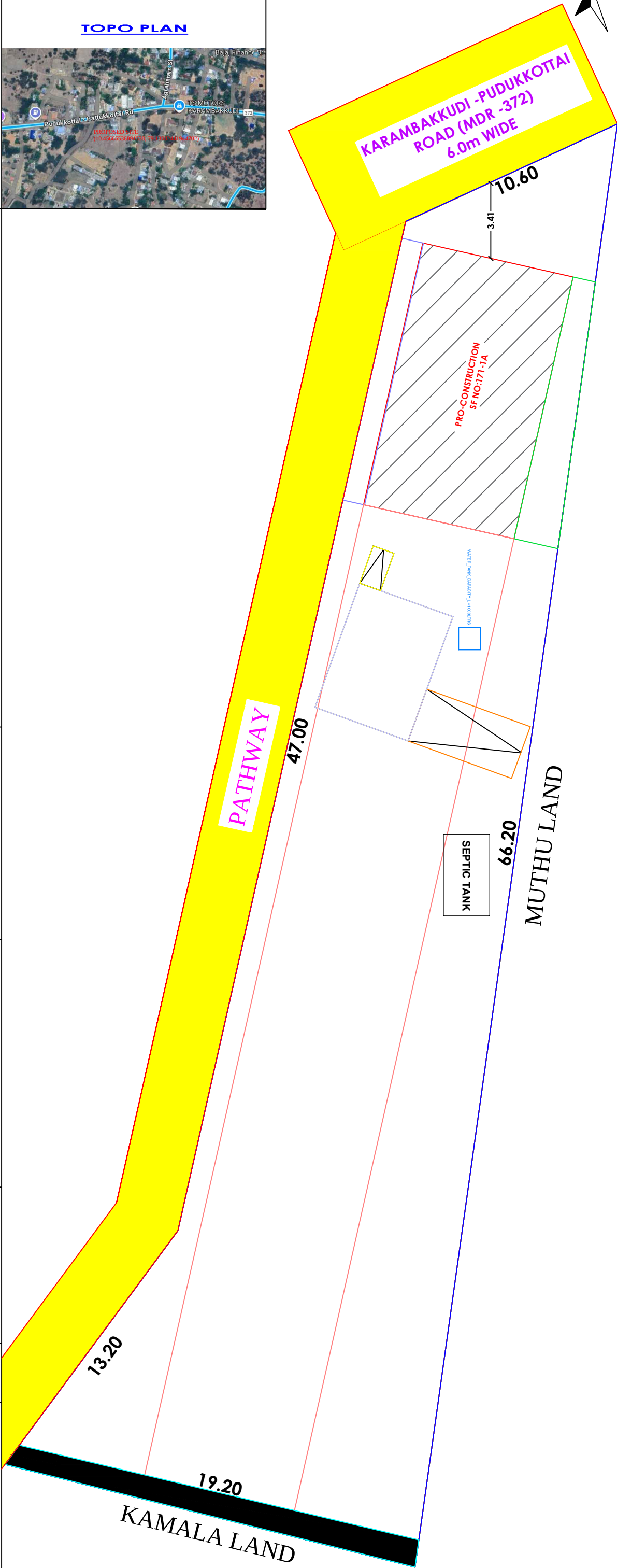
SITE PLAN
