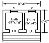
PLAN OF TOILET BLOCK
