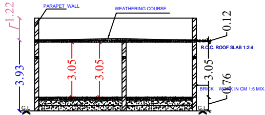
Section on-"AA"
