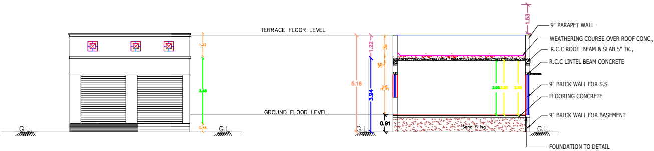
FRONT ELEVATION
