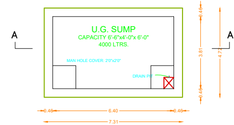
SUMP DETAIL
