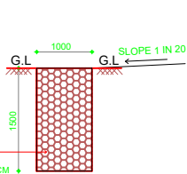
SECTION OF PEBBLE TRENCH SCALE: 1: = 100
