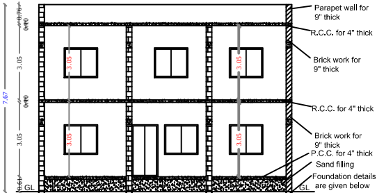
SECTION "AA & BB"
