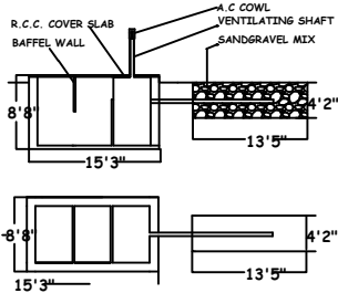
SEPTIC TANK AND DISPERSION TRENCH DETAILS
