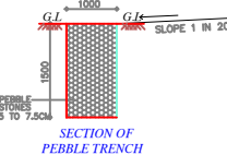
SECTION OF PEBBLE TRENCH
