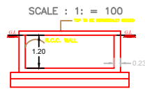
SCALE : 1: = 100 RWL_CAPACITY_L = 2000LTRS
