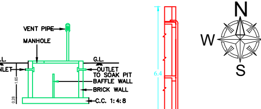
SECTION OF SEP.TANK
