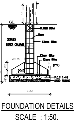
FOUNDATION DETAILS
