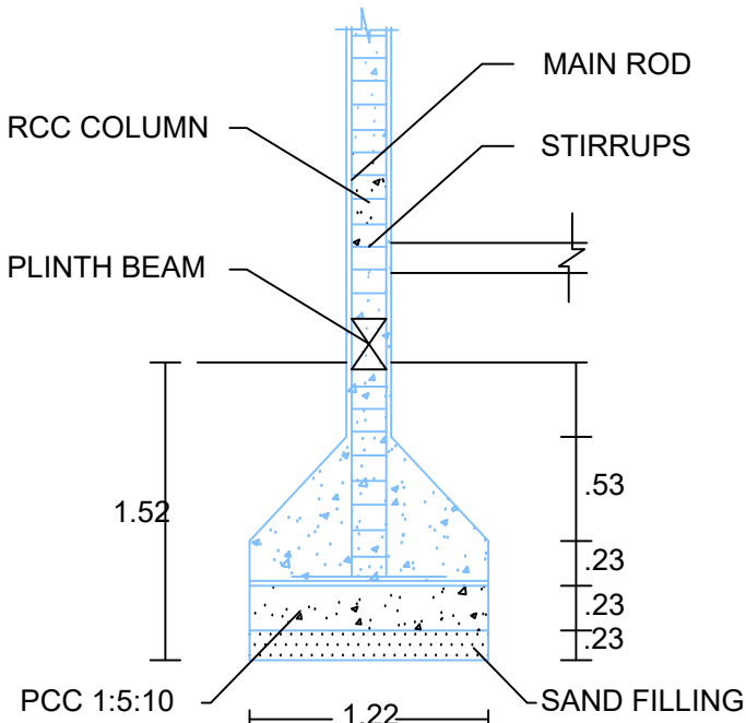
COLUMN DETAILS
