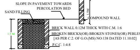
SECTION OF RAIN WATER PERCOLATION BED
