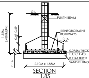
FOUNDATION DETAILS
