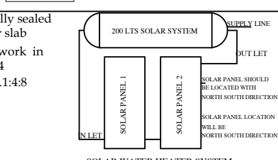
SOLAR WATER HEATER SYSTEM
