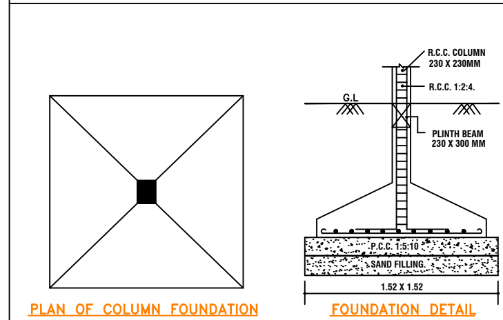
PLAN OF COLUMN FOUNDATION
