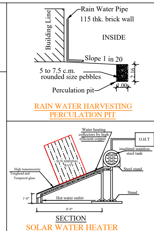
SOLAR WATER HEATER
