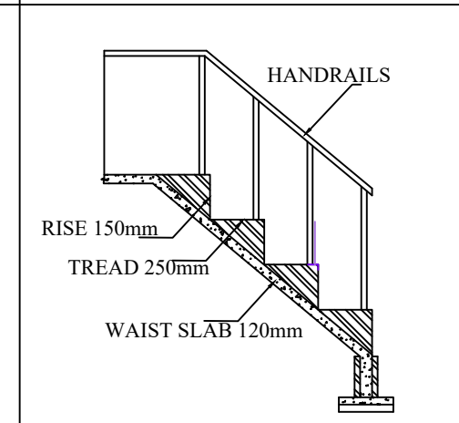
STAIRCASE DETAILS
