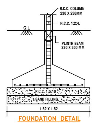
FOUNDATION DETAIL
