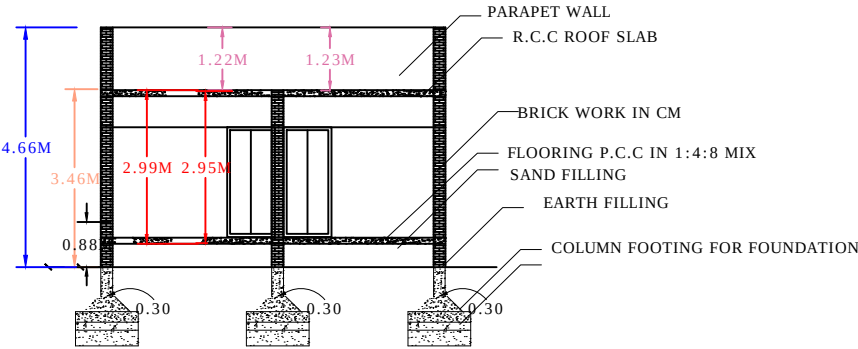
SECTION "AB"
