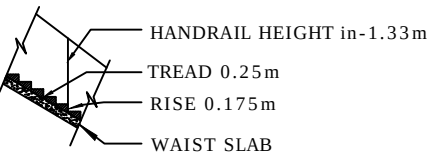
STAIRCASE DETAILS
