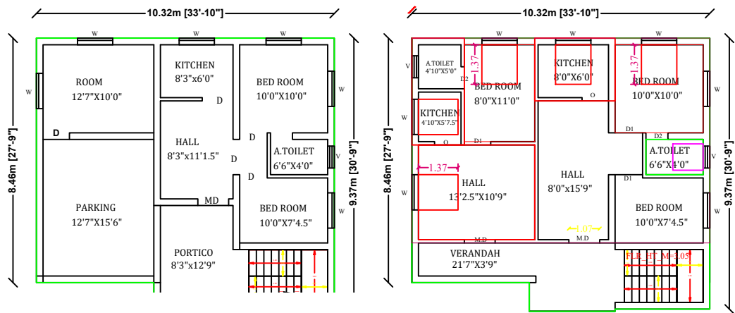
PRO-FIRST FLOOR PLAN
