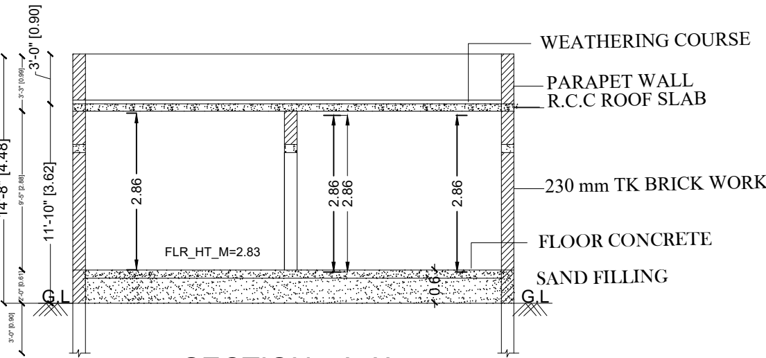
SECTION - A,A'
