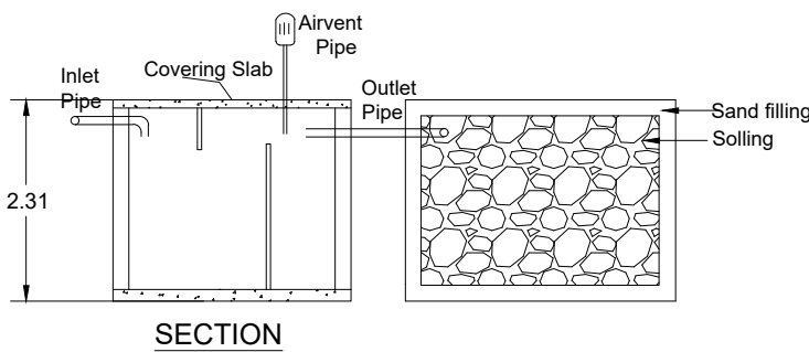
SECTION
