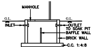
SECTION OF SEP.TANK
