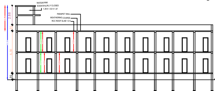
SECTION 'A-B'
