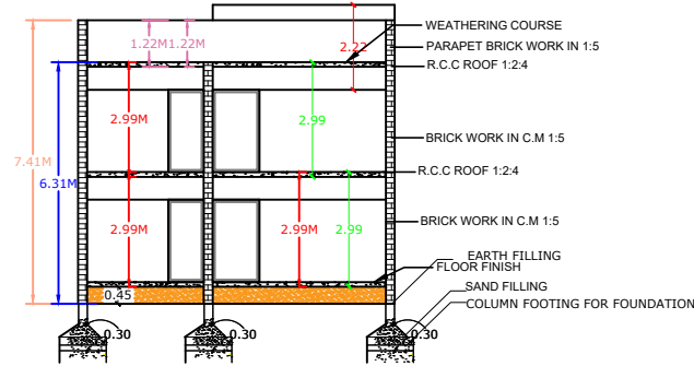
SECTION "AB"
