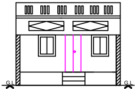
Front Elevation
