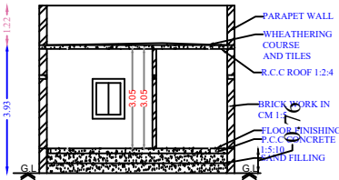
Section on-"AA"
