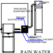
RAIN WATER
