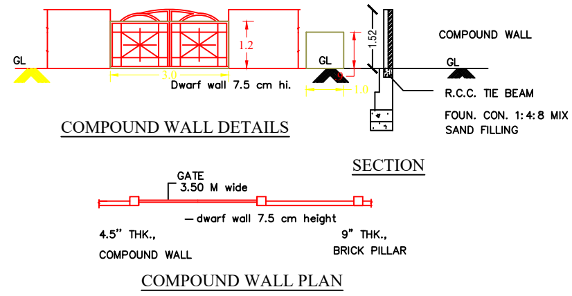
SCALE 1: 100
