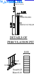
STAIRCASE DETAIL
