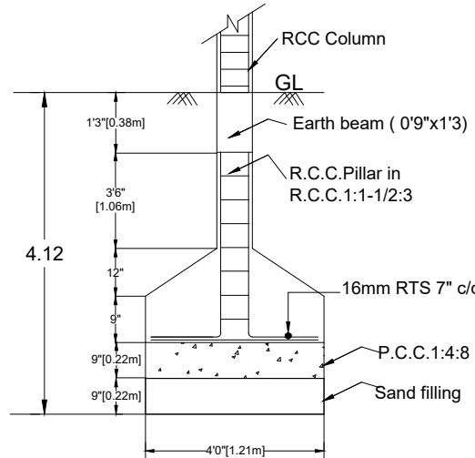
FOUNDATION DETAILS
