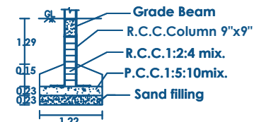
COLUMN DETAILS
