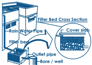
DETAILS OF RWH
