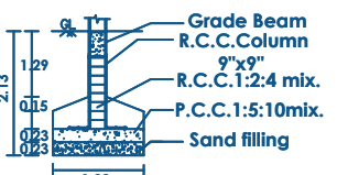
COLUMN DETAILS
