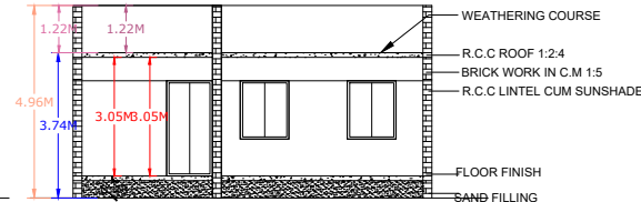
SECTION "XX"
