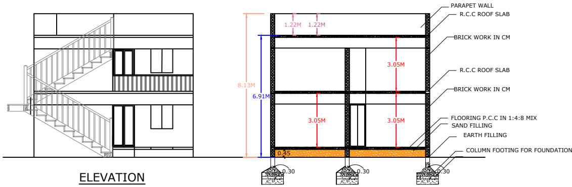
SECTION "AB"
