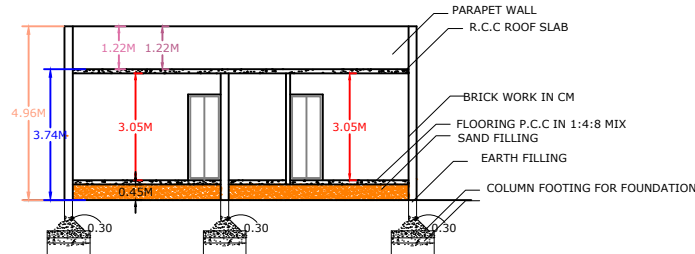
SECTION "AB"
