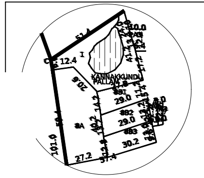
TOPO PLAN
