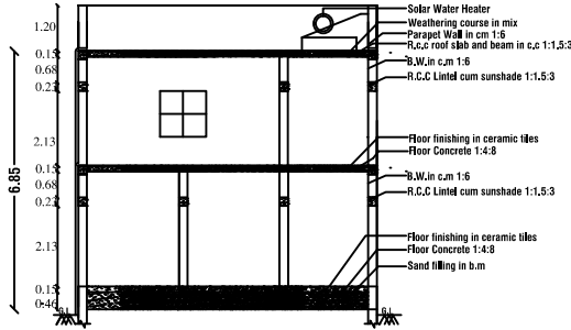
SECTION - "AB"
