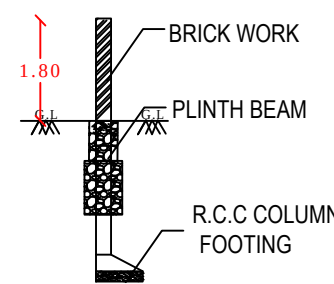
SECTION
