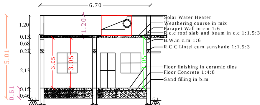
SECTION - "AB "
