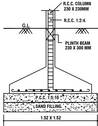
FOUNDATION DETAIL
