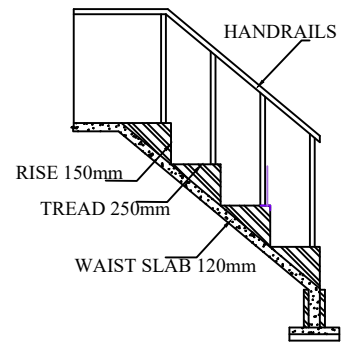
STAIRCASE DETAILS
