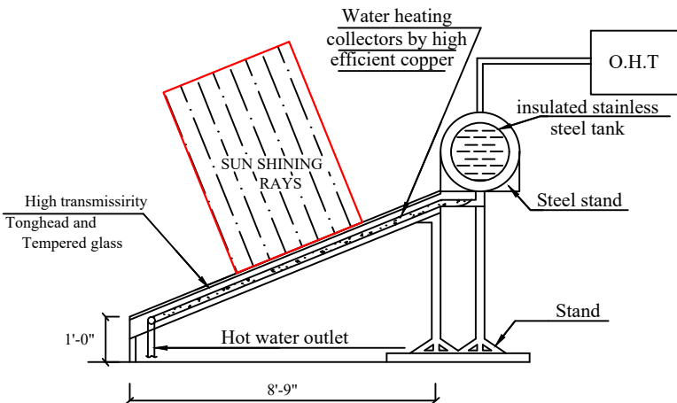
SECTION SOLAR WATER HEATER
