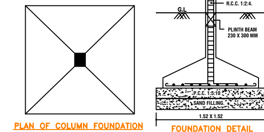
PLAN OF COLUMN FOUNDATION
