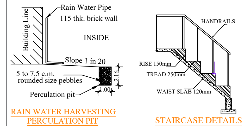
STAIRCASE DETAILS
