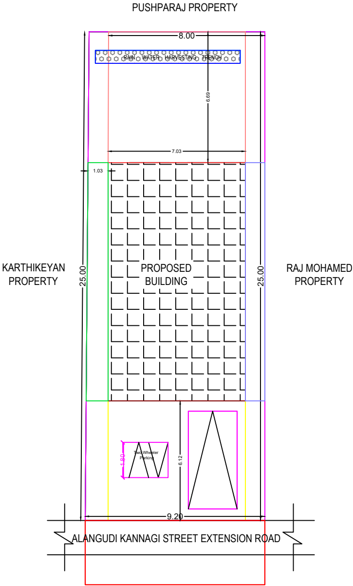
SITE PLAN (1:100)
