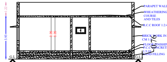
Section on-"AA"
