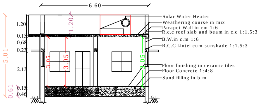
SECTION - "AB "
