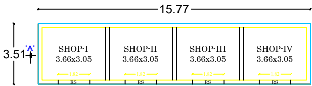
GROUND FLOOR PLAN BLOCK-II (COMMERCIAL)
