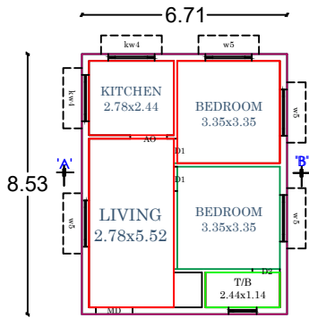
GROUND FLOOR PLAN BLOCK-I (RESIDENTIAL)
