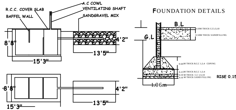
SEPTIC TANK AND DISPERSION TRENCH DETAILS
