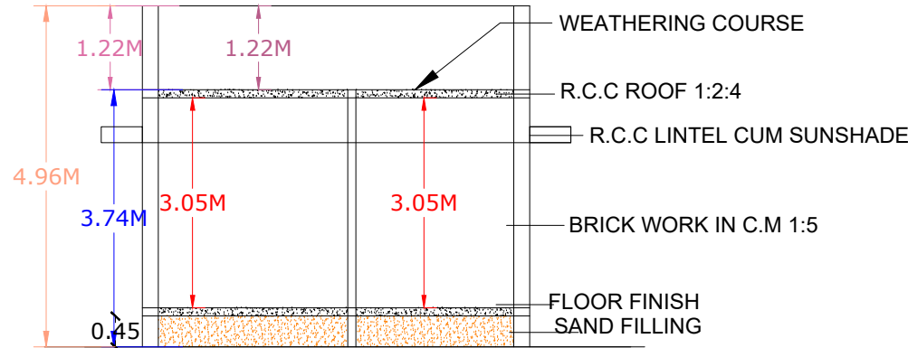
SECTION "AB"
