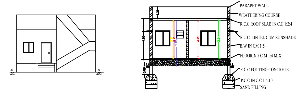
ELEVATION 6.70
