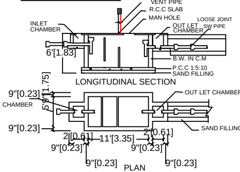
SEPTIC TANK:
