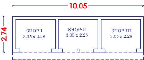
GROUND FLOOR PLAN COMMERCIAL (SHOP) BUILDING BLOCK - I
