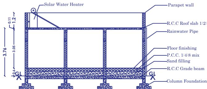
SECTION ON "AB" BLOCK - I
