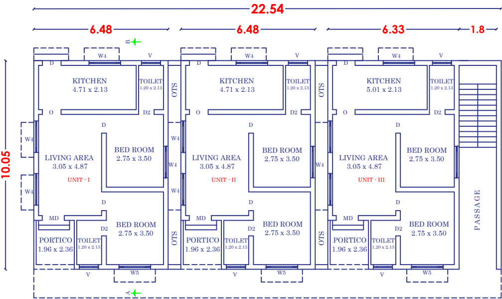
GROUND FLOOR PLAN RESIDENTIAL BUILDING BLOCK - II
