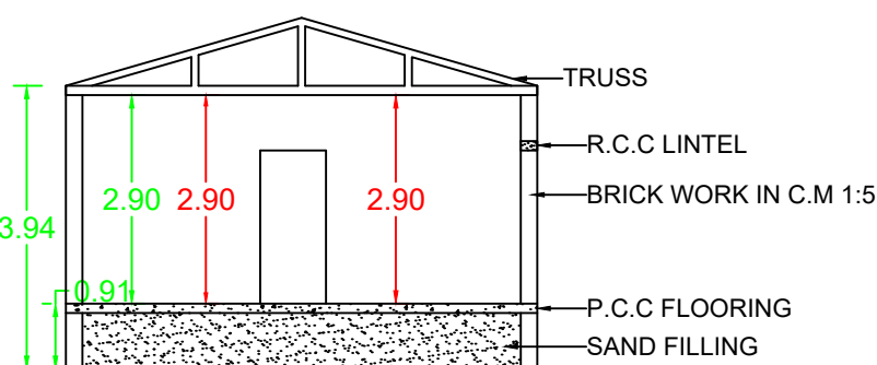
BLOCK - 1 SECTION ON A-A
