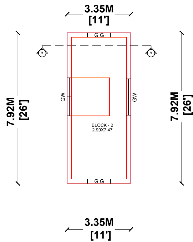
BLOCK - 2 PROPOSED GROUND FLOOR PLAN
