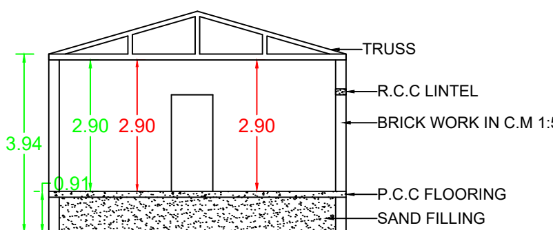
BLOCK - 2 SECTION ON A-A
