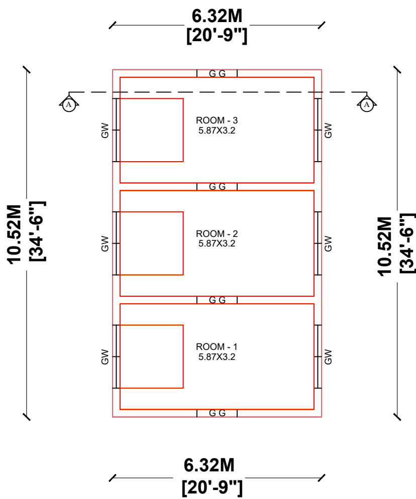
BLOCK - 1 PROPOSED GROUND FLOOR PLAN
