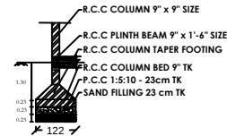
SECTION COLUMN DETAILS PLAN
