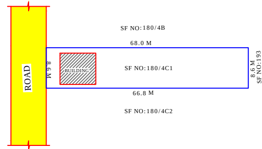
SITE PLAN (NOT TO SCALE)
