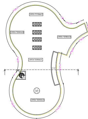
TERRACE FLOOR PLAN (BLOCK-6)
