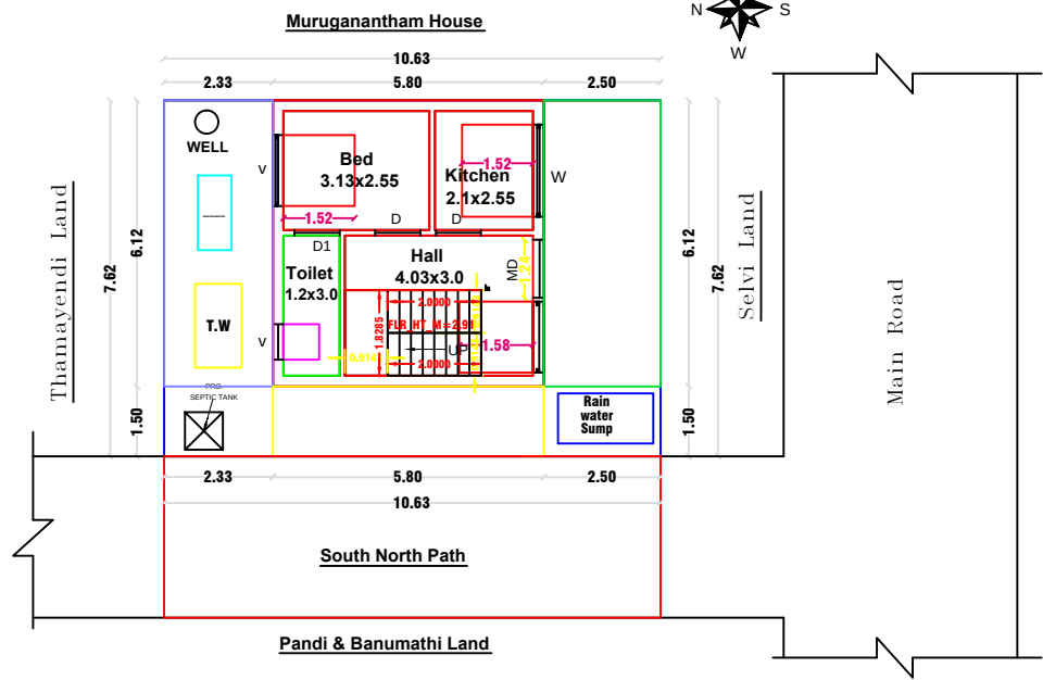
SITE PLAN CUM GROUND FLOOR PLAN
