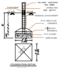
FOUNDATION DETAIL
