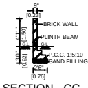
SECTION - CC
