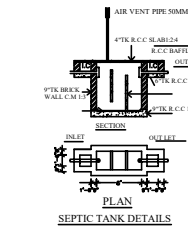
SEPTIC TANK DETAIL
