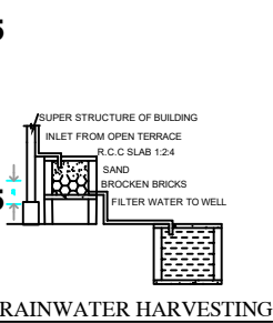
RAINWATER HARVESTING
