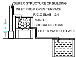
RAINWATER HARVESTING
