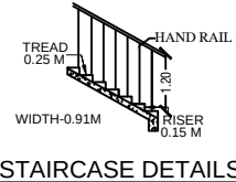
STAIRCASE DETAILS
