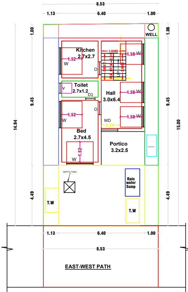
SITE PLAN CUM GROUND FLOOR PLAN
