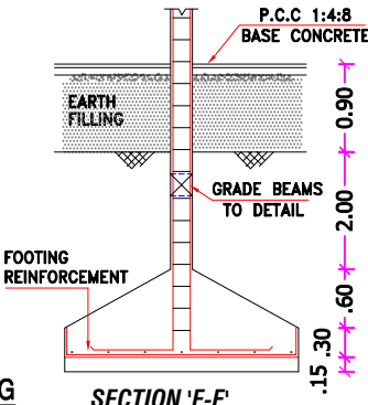
SECTION 'E-E'
