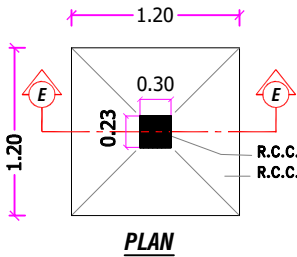
DETAILS OF COLUMN FOOTING
