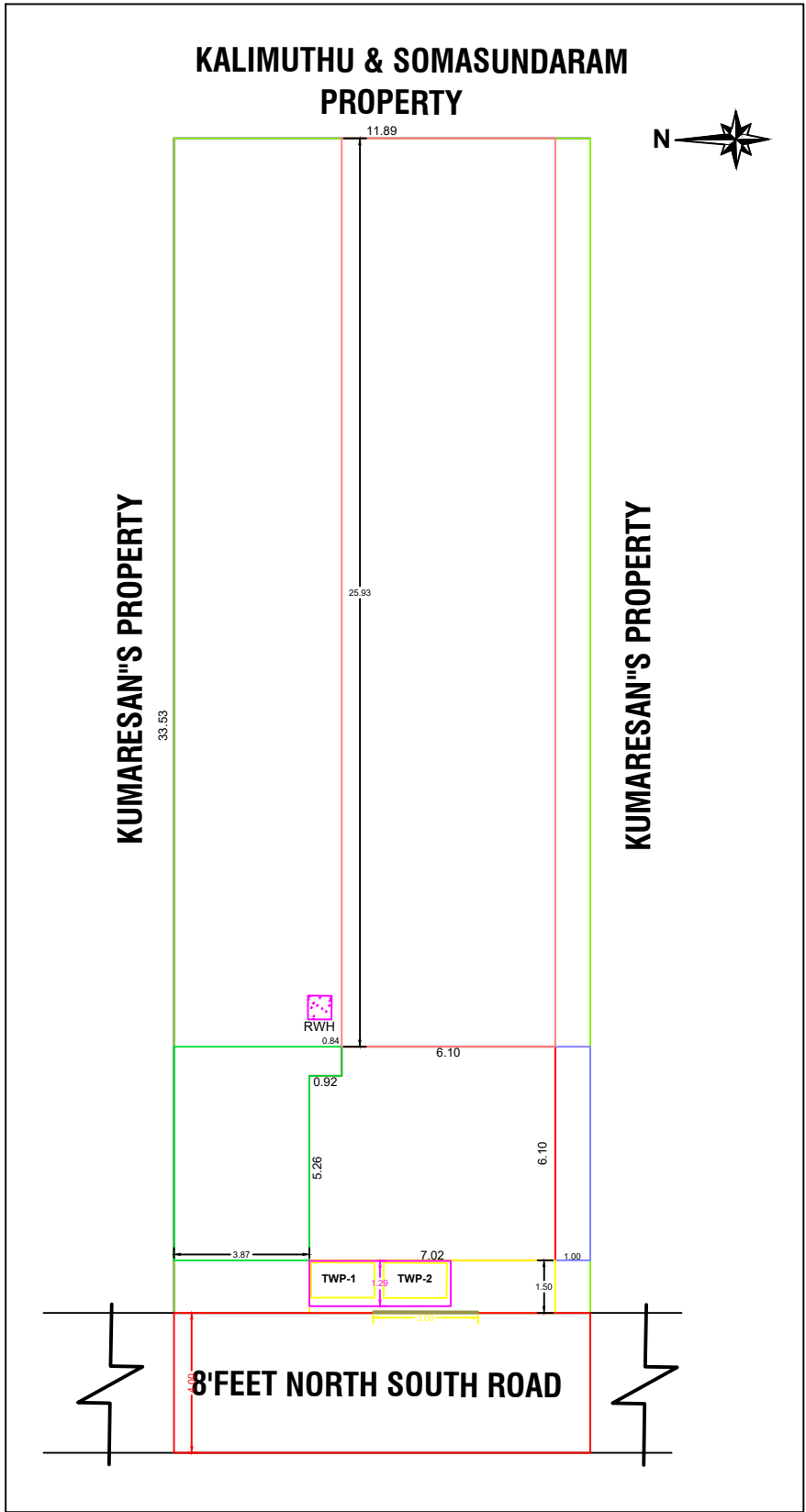
SITE PLAN
