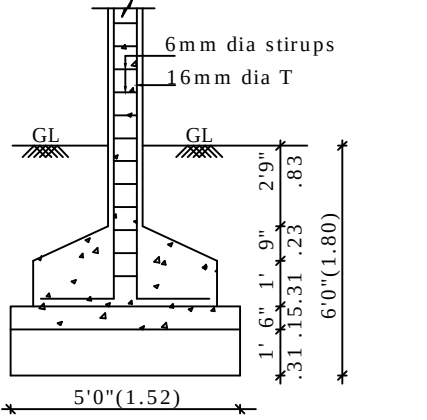
COLUMN FOUNDATION DETAIL
