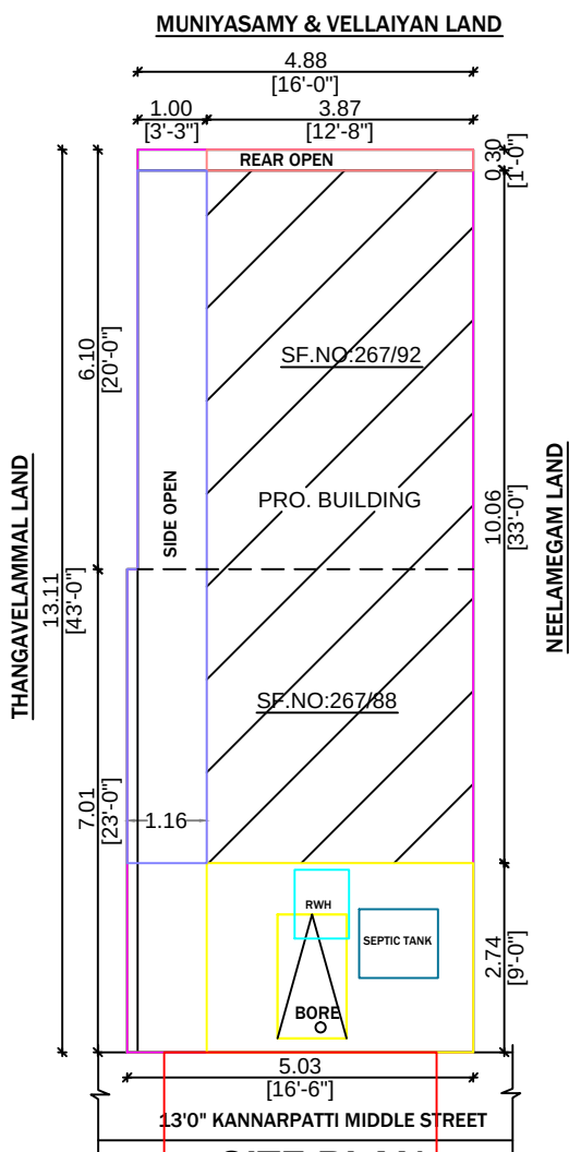
SITE PLAN
