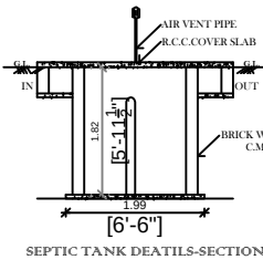
SEPTIC TANK DEATILS-SECTION
