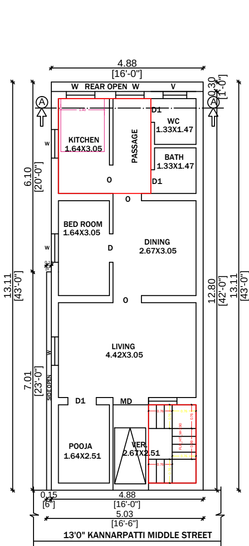
EXG. GROUND FLOOR PLAN
