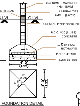
FOUNDATION DETAIL
