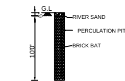
PERCOLATION PIT
