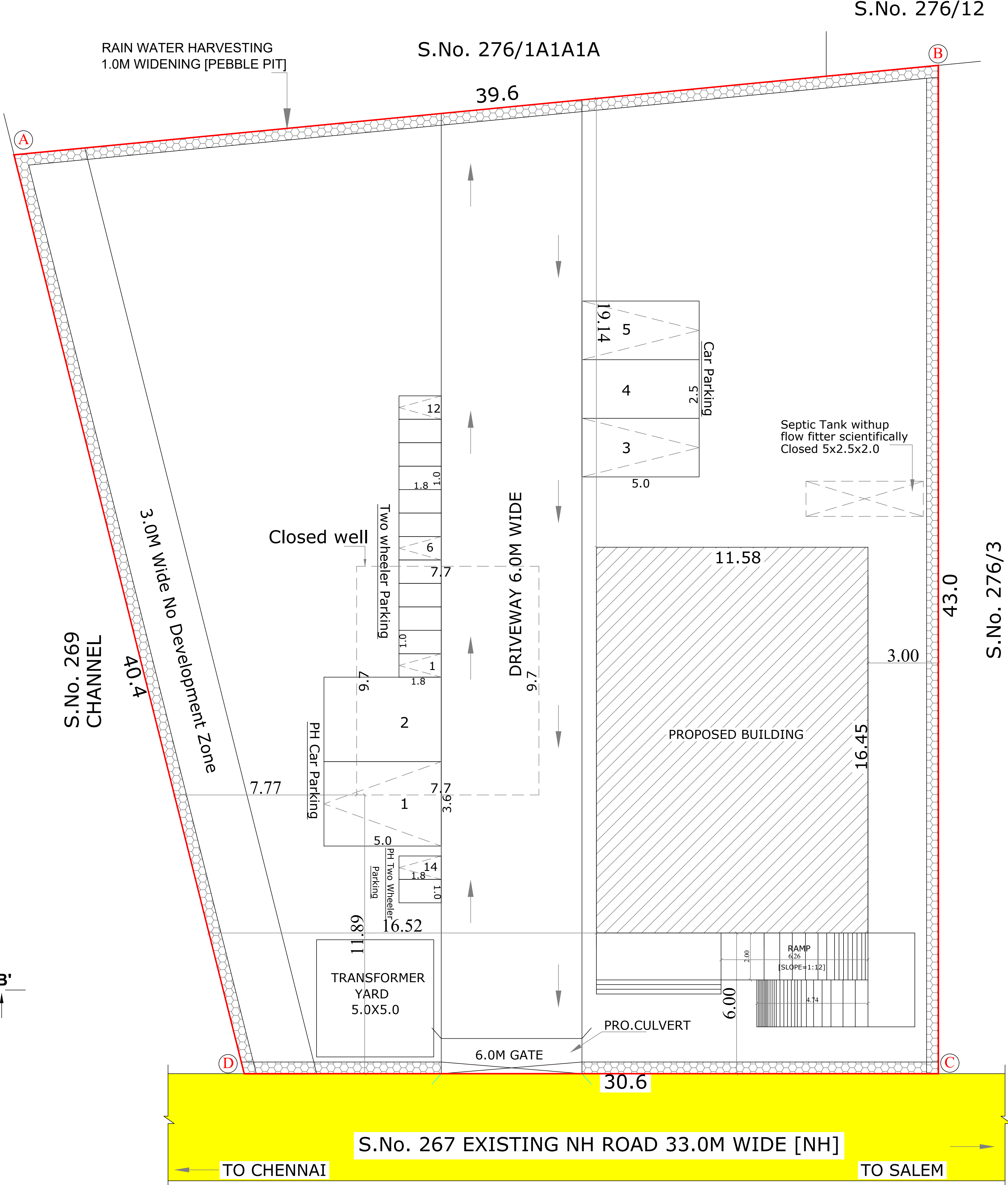
SITE PLAN
